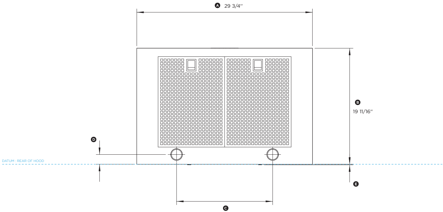
BOTTOM VIEW
