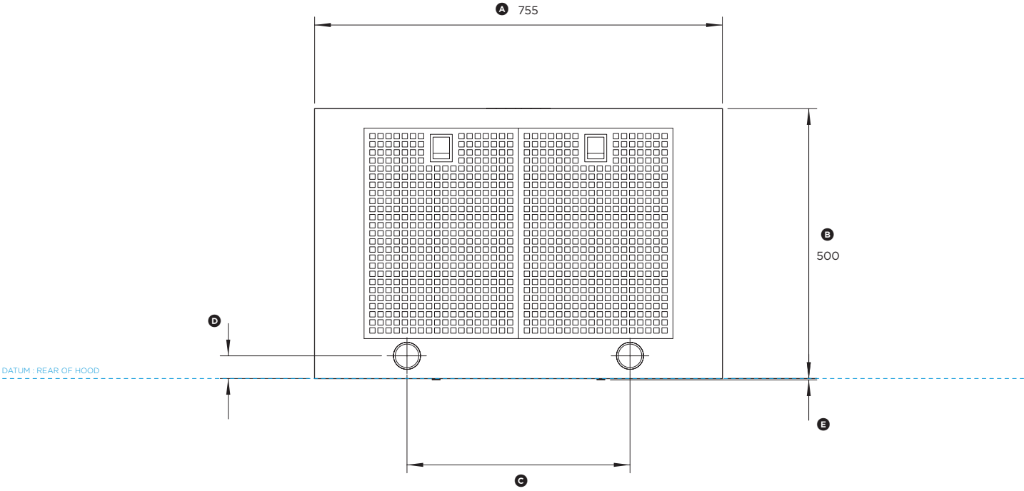
BOTTOM VIEW
